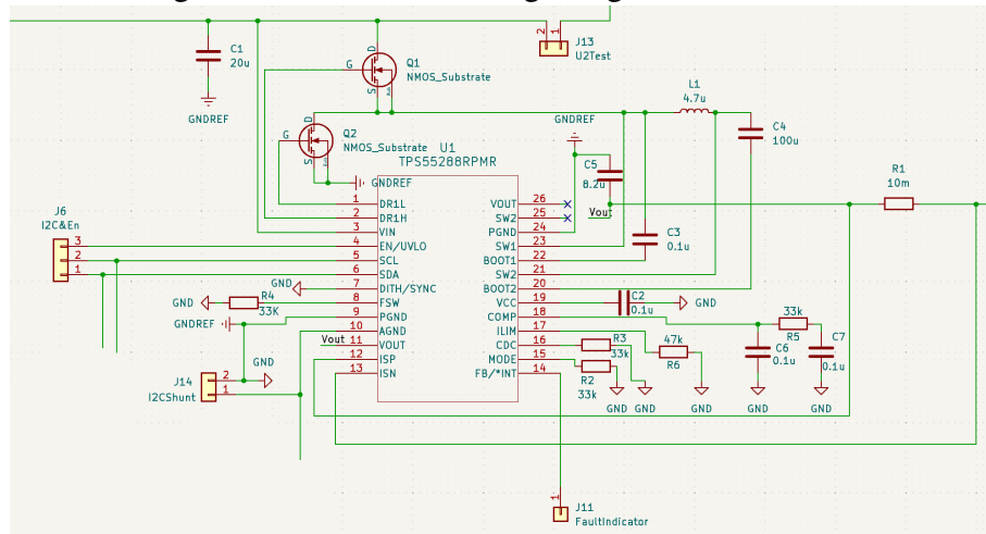
Fig. 7: TPS55288RPMR Buck-Boost Schematic
